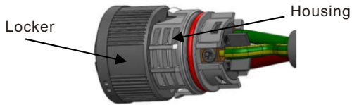
Figure 4.7 Connect Wires to the Terminal
