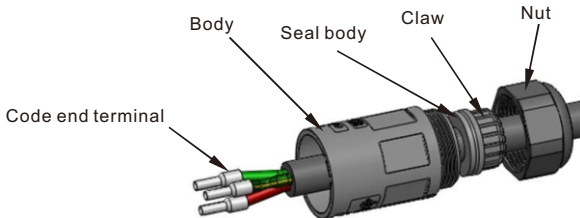
Figure 4.5 AC Grid Terminal Connector
