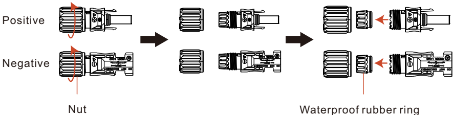
Figure 4.11 Remove the cover of the terminal connector
