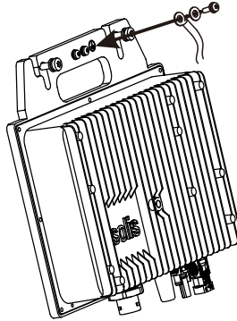
Figure 4.3 Connect the external grounding conductor
