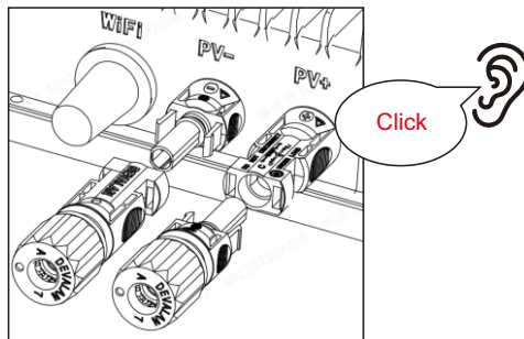
Figure 4.16 connect to the inverter
