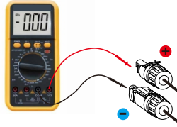
Figure 4.15 multi-meter measurement
